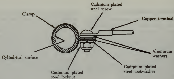
A. Copper jumper connection to tubular structure.
